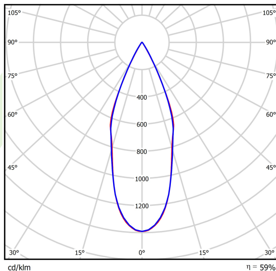
cd/klm — C0 - C180 — C90 - C270 \eta = 59\%
