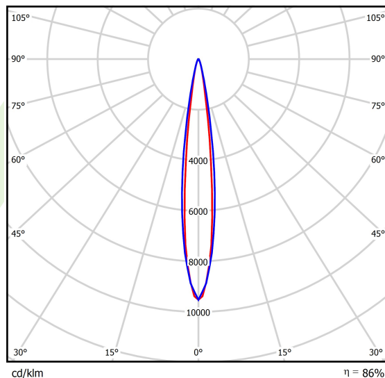
cd/klm — C0 - C180 — C90 - C270 \eta = 86\%
