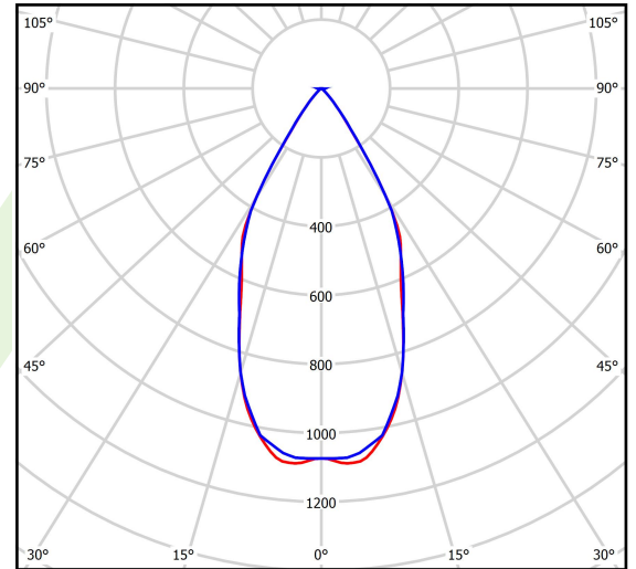
cd/klm — C0 - C180 — C90 - C270 η = 76%
