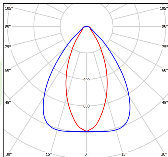
cd/klm — C0 - C180 — C90 - C270 η = 95%
