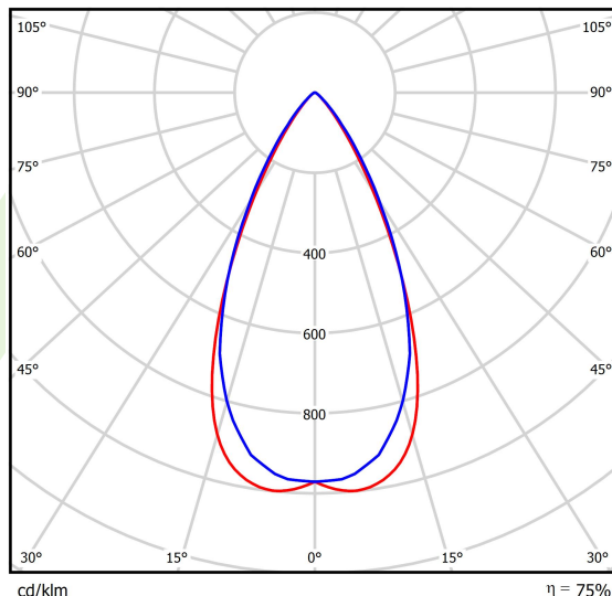
cd/klm — C0 - C180 — C90 - C270 η = 75%
