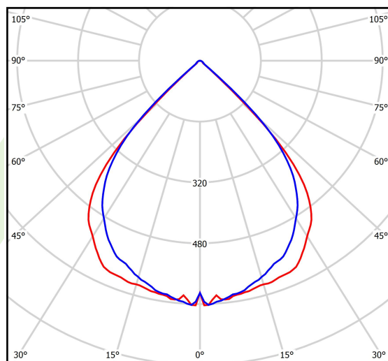
cd/klm — C0 - C180 — C90 - C270 \eta = 96\%
