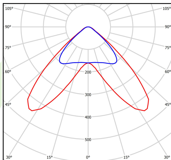
cd/klm \eta = 92\% — C0 - C180 — C90 - C270
