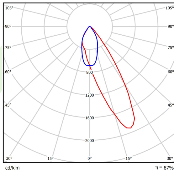
cd/klm — C0 - C180 — C90 - C270 η = 87%
