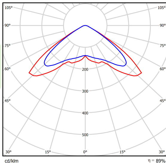
cd/klm — C0 - C180 — C90 - C270 η = 89%
