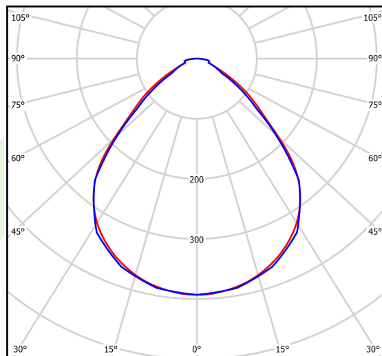
cd/klm — C0 - C180 — C90 - C270 η = 83%
