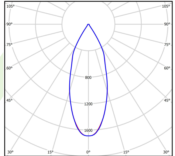
cd/klm — C0 - C180 — C90 - C270 η = 86%
