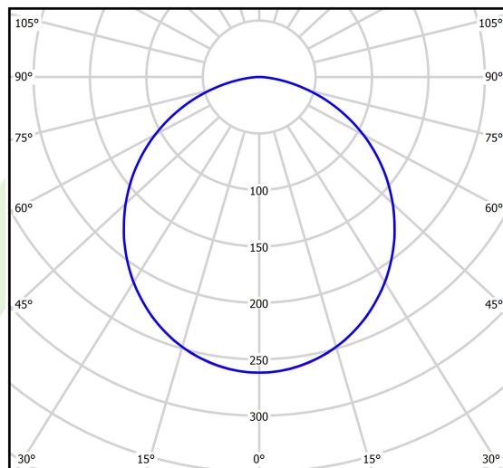
cd/klm — C0 - C180 — C90 - C270 η = 72%
